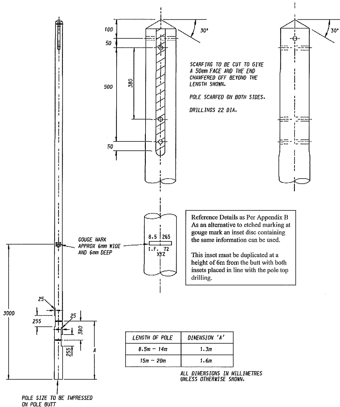
OH4T Fig 1 - Single Pole Drillings, Scarfing & Marking
